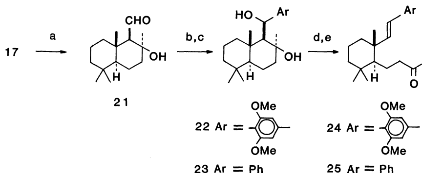
Scheme 2. (a) NCS, Me 2 S, toluene (63%); (b) 1,3-dimethoxy-5-methylbenzene ( 26 ), BuLi, DME (92%); (c) PhLi, DME (90%); (d) Py·HCl or PPTS, CH 2 Cl 2 , rt, a few minutes (quant); (e) p -TsCl, Py, 60 °C, 2d (58%).
